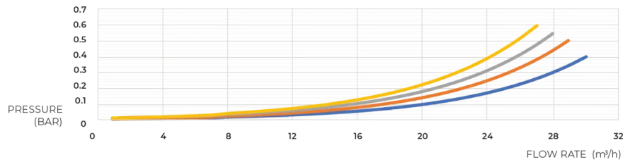
PRESSURE DROP SECONDARY CIRCUIT
