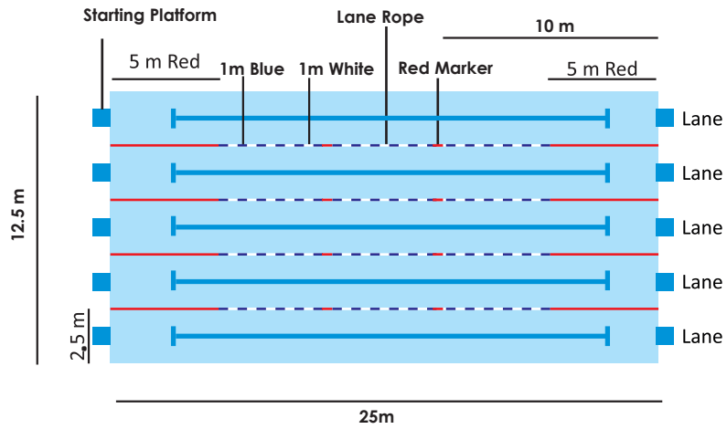
SWIMMING POOL RACING LANE MARKING TYPE – TRAINING POOL
