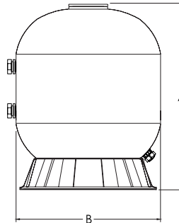
RO-400N-VS/ 525 / 625
