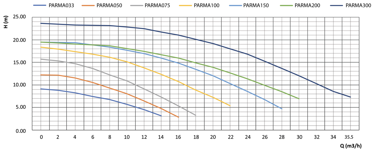
PARMA - PERFORMANCE CURVE
