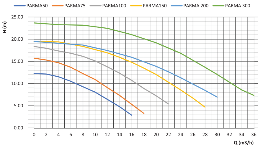
PARMA - PERFORMANCE CURVE
