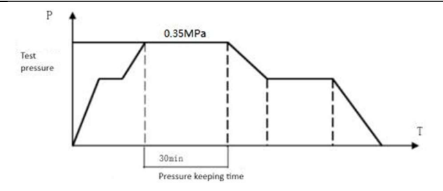
Design requirement pressure test curve
