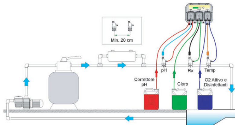
INSTALLATION EXAMPLE - TECHNOPOOL 3
