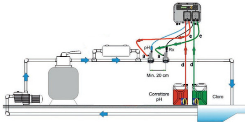
INSTALLATION EXAMPLE - TECHNOPOOL 3
