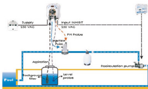
INSTALLATION EXAMPLE-PH
