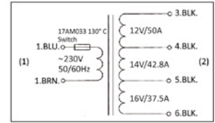
E-248 CIRCUIT DIAGRAM
