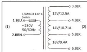
E-245 CIRCUIT DIAGRAM
