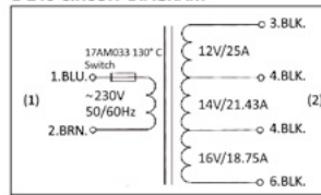
E-246 CIRCUIT DIAGRAM
