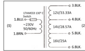
E-247 CIRCUIT DIAGRAM
